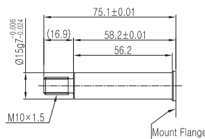
THREAD (JIS)
