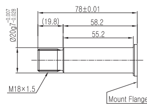
THREAD (JIS)
